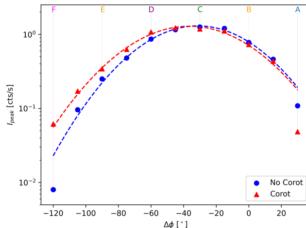
Fig. 4. Peak intensity versus \Delta\phi for the six observers A-F with (red triangles) and without (blue circles) the effects of corotation for scattering conditions described by \lambda = 0.1 au. The points are fit with Gaussian functions shown as the dashed lines.
